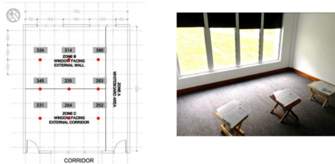
Figure 4: Classroom PNP-A1-001 Illuminance Measurement Point (Source: Raja Syaheeza, 2020)
