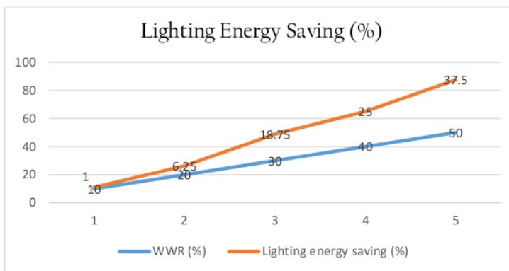
Figure 11. Lighting energy saving based on WWR
