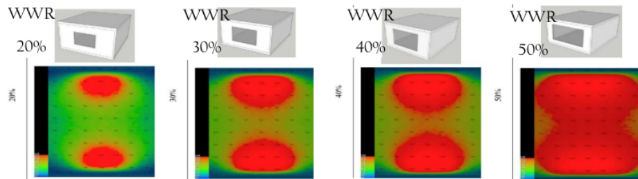
Figure 8. Result of Illuminance level based on WWR (percentage)
