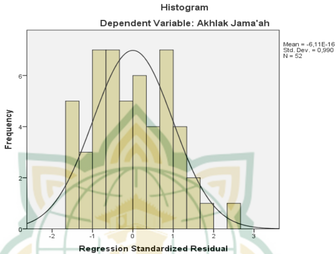
Gambar 4.2 Normal Plot
