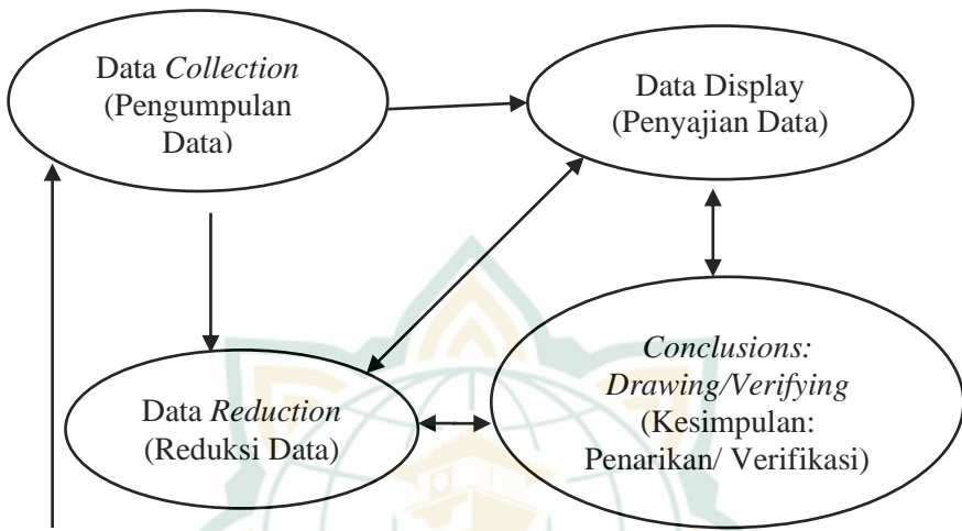
Gambar 3.1 Alur Penelitian
